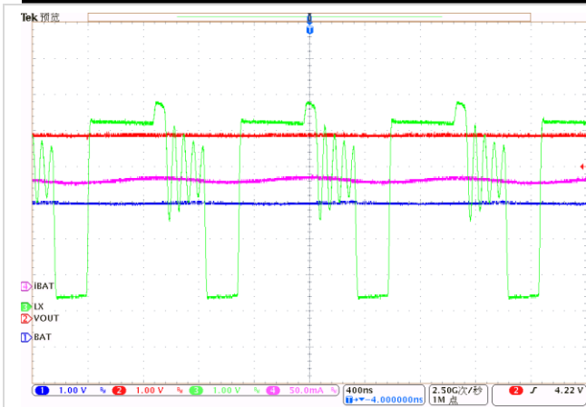
Boost, IOUT=100mA
